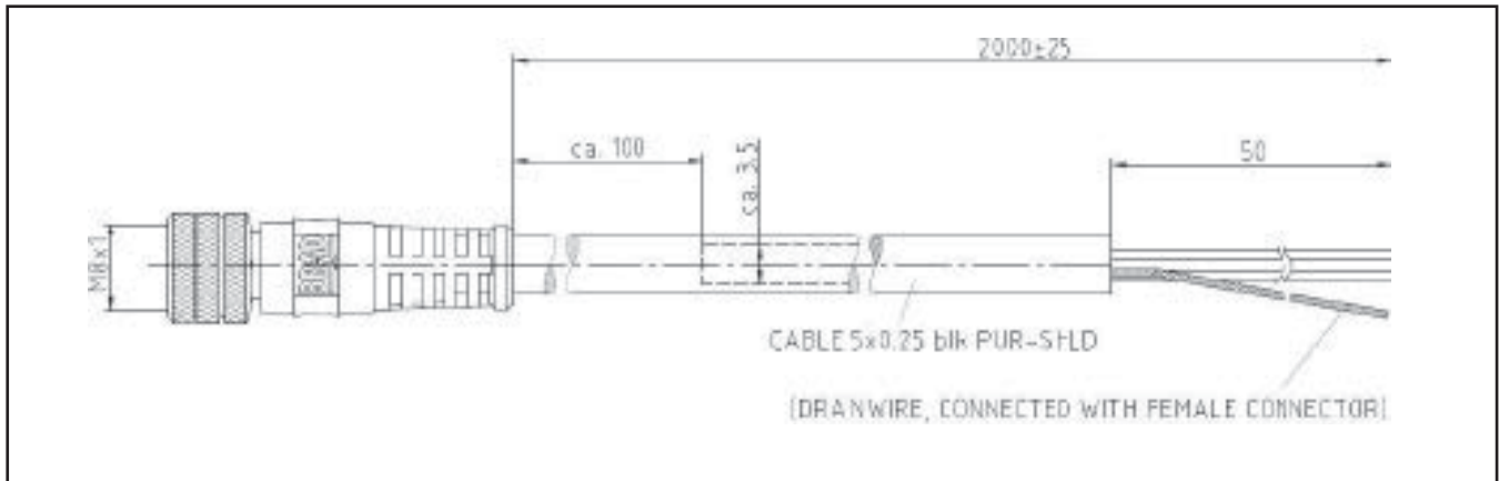
Figure 4-6: M8 Female Mating Cable
