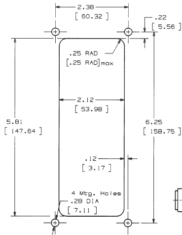
Flush panel mounting with bezel
