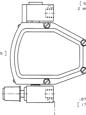
2 mounting holes 10-32 unf x .25" Deep [6,35]
