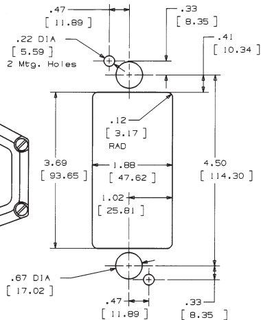
Front of panel mounting
